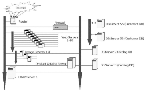
Figure 2: Simplified configuration of the B2C site.
