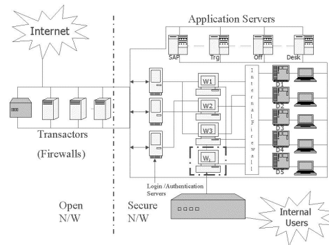
Figure 3: Simplified configuration of the B2B site.
