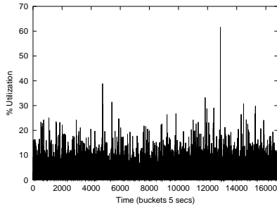
Figure 7: Processor(2P) Utilization of one of the front-end web-servers at B2B site
