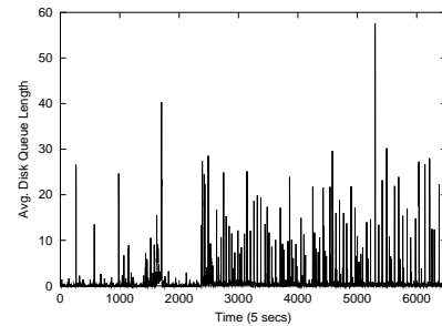
Figure 16: Disk Queue Length at Main DB server (5sec)
