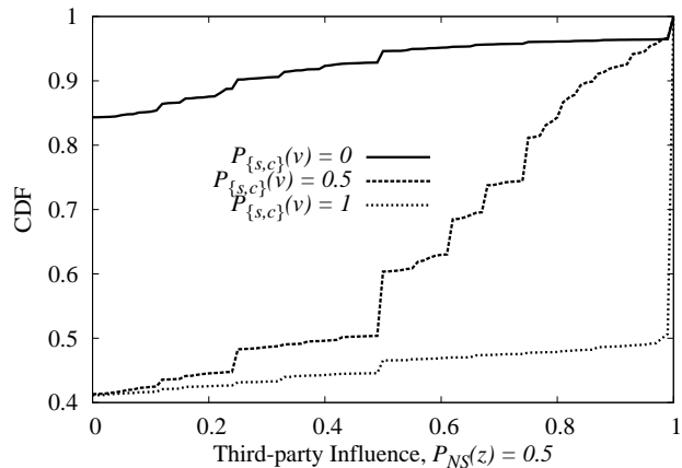
Fig. 9. The CDF for the third-party influence of the ODP/SC08 hostnames, grouped by zone.
