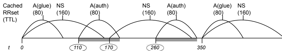
Fig. 12. A timeline of queries to a resolver for names within a particular zone and which are not found in the resolver’s cache. The labels on top of the timeline indicate the cache lifetimes of the NS RRset for the zone and the A RRset from the glue and authoritative answers. The ticks on the bottom mark the times at which queries for uncached names in the zone arrive at the resolver, inducing queries for NS or A RRsets, as appropriate. Queries at the circled times represent queries for authoritative A RRsets, and shading along the bottom of the timeline highlights the time in which authoritative A RRsets exist in cache.
