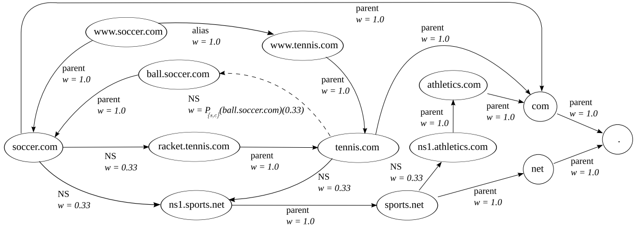
Fig. 3. The dependency graph for the domain name www.soccer.com , derived from the zone data in Table I. The solid lines represent active influence, and the dashed lines represent passive influence.
