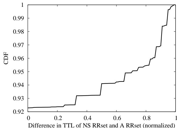
Fig. 13. The CDF showing the normalized difference between NS and A RRsets for NS-type dependencies in the data seeded by the ODP/SC08 names.
