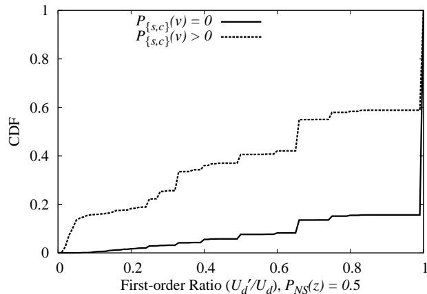
Fig. 8. The CDF for the first-order ratio of the ODP/SC08 hostnames.
