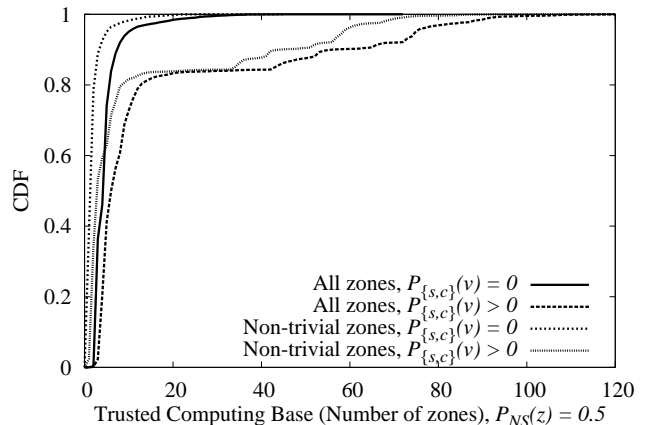
Fig. 7. The CDF for the size of the TCB of ODP/SC08 hostnames. Included are the CDF for the number non-trivial and total zones in the TCB, for P_{\{s,c\}}(v) = 0 and P_{\{s,c\}}(v) > 0 .
