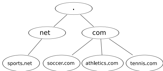
Fig. 1. The zone hierarchy for the the zone data shown in Table I.
