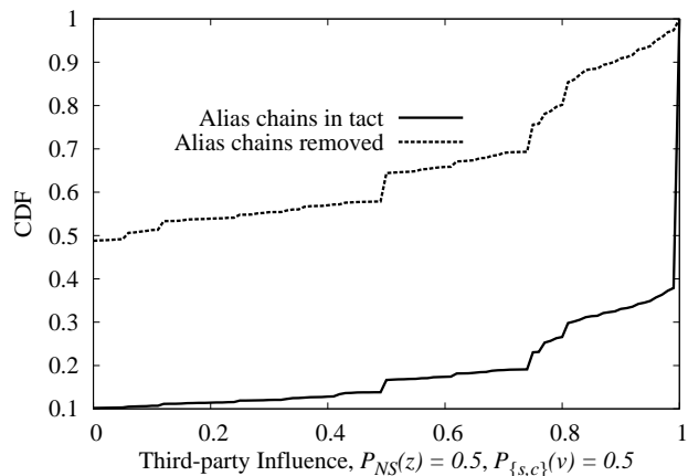
Fig. 10. The CDF for the third-party influence of ODP/SC08 hostnames affected by alias chains, grouped by zone.
