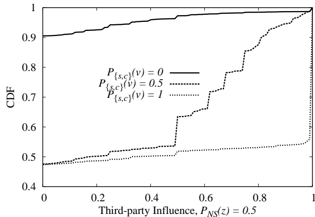
Fig. 11. The CDF for the third-party influence of ODP/SC08 hostnames, grouped by organization.
